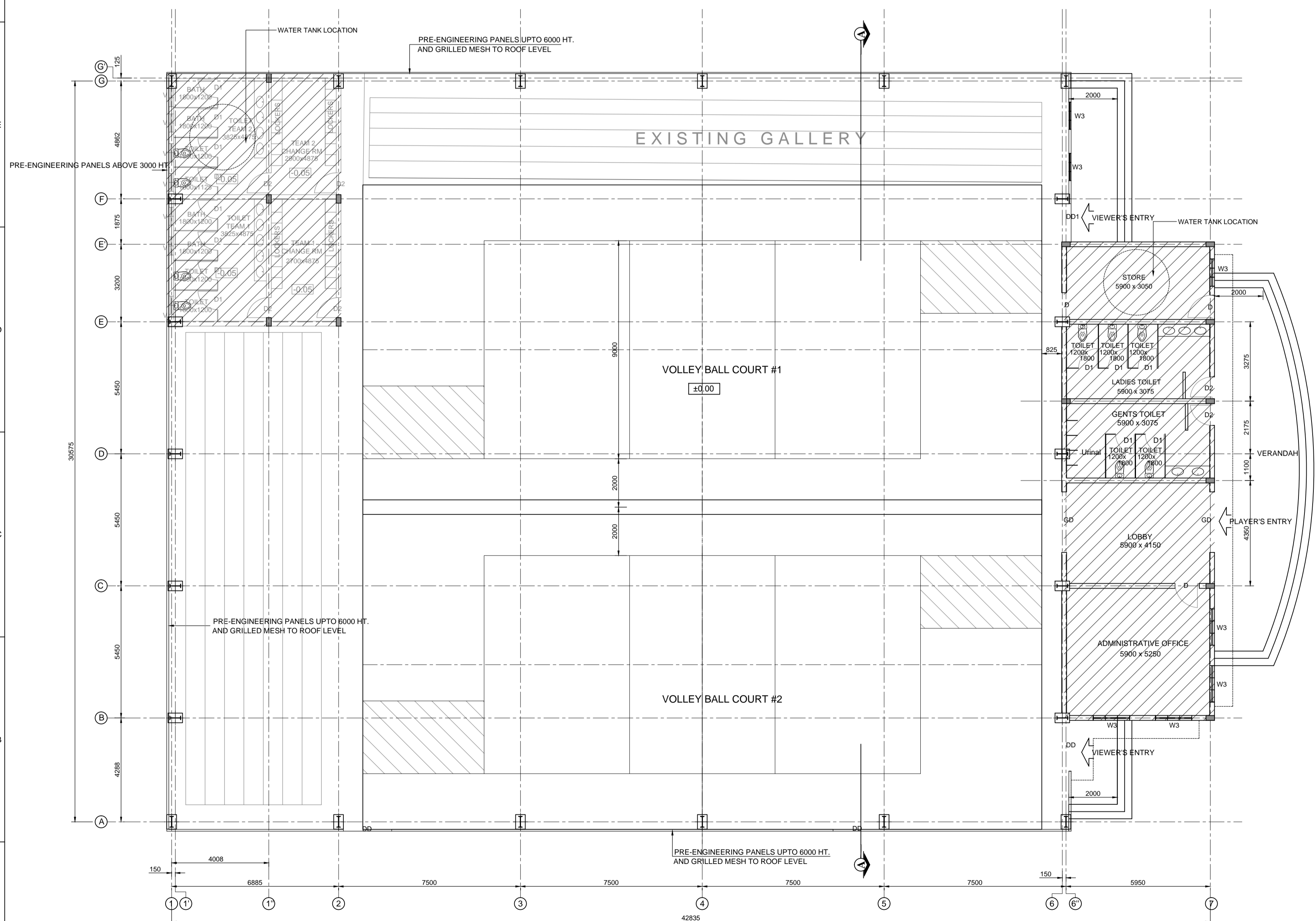
PLAN (Plinth Area : 1283.00 Sq.M)
