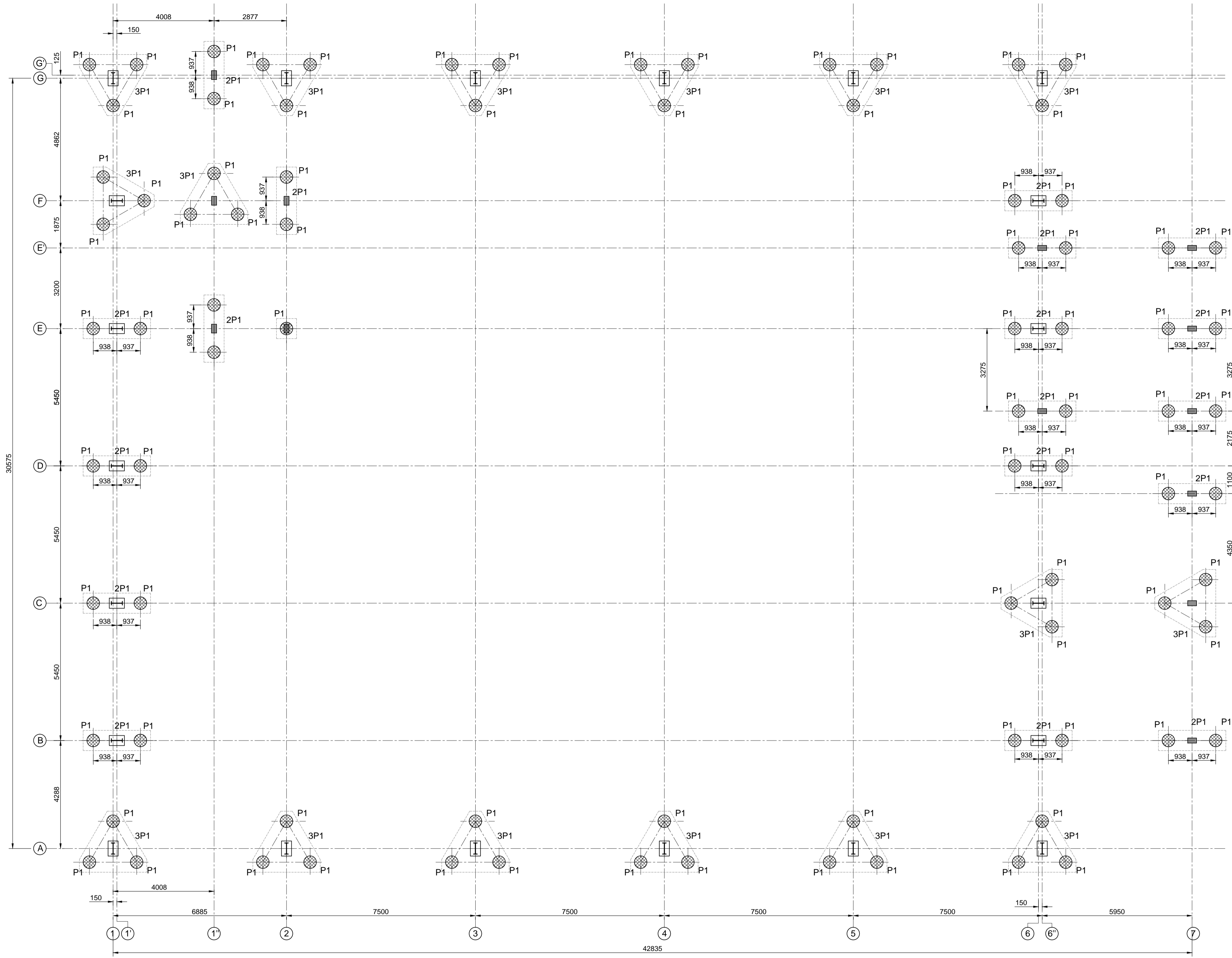
PILE LAYOUT
