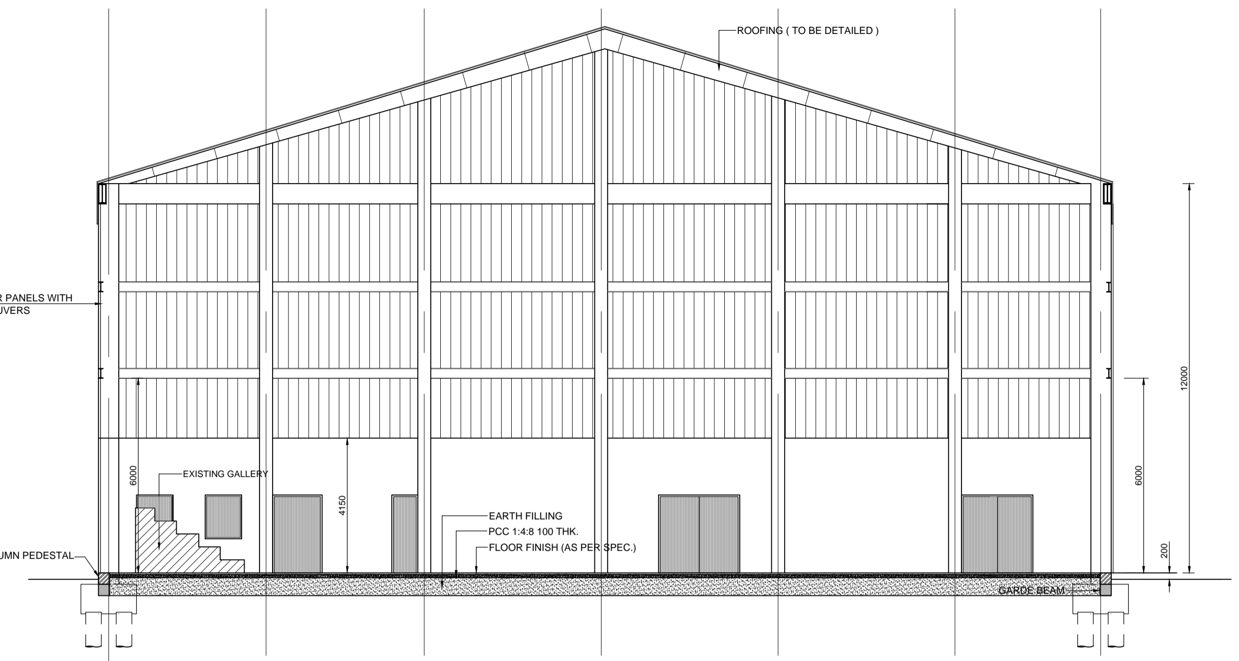
SECTION - AA
