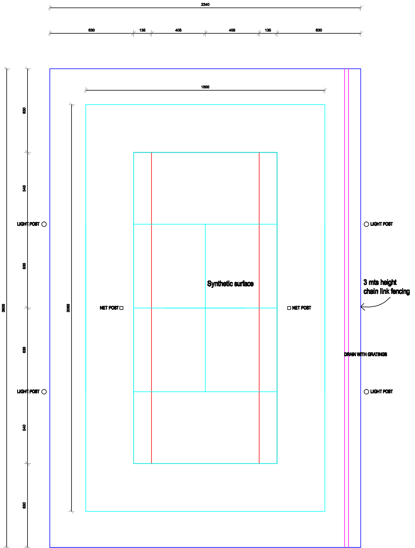
TENNIS COURT 36 m x 23.40 m
