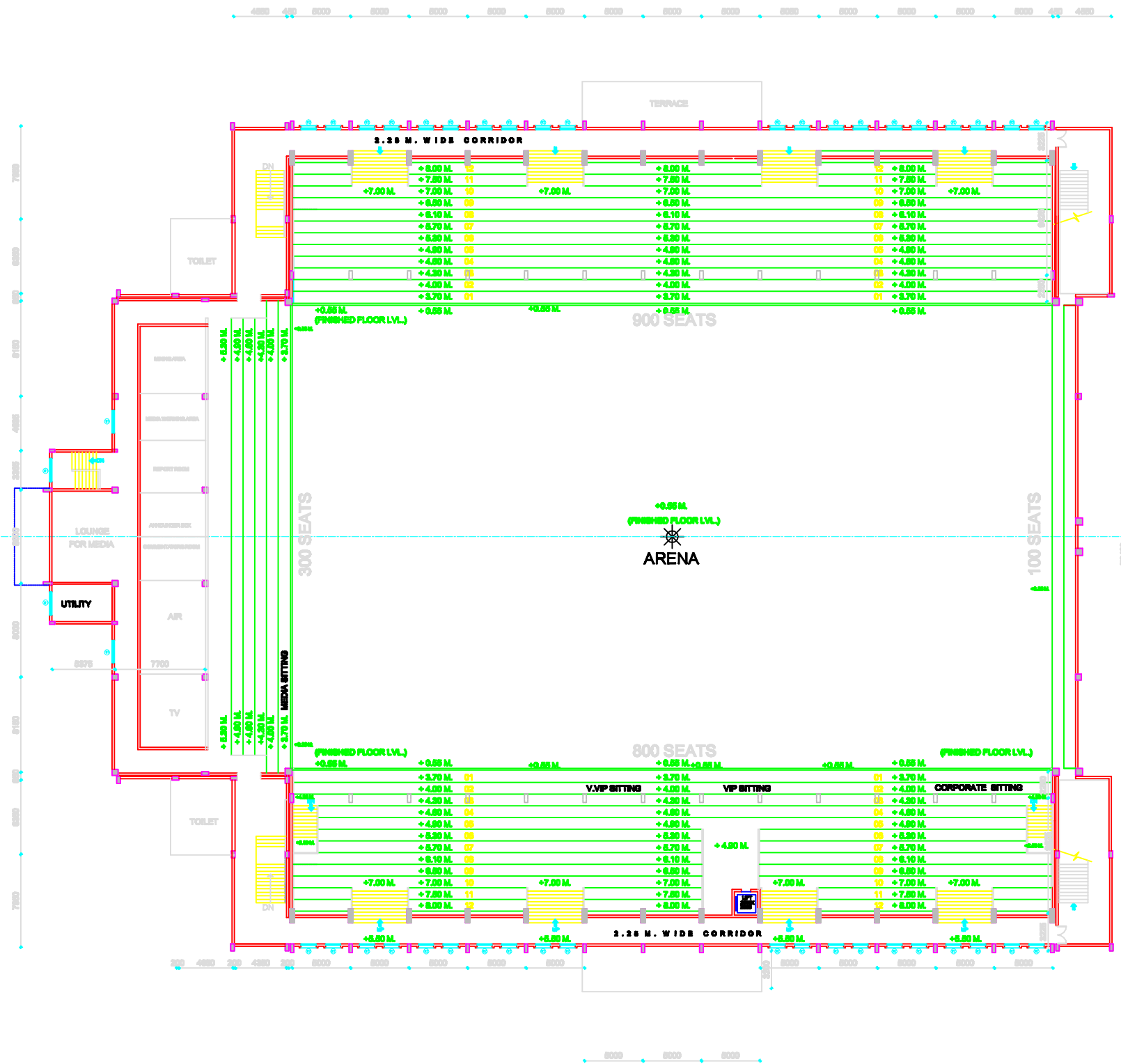
FIRST FLOOR LEVEL PLAN
