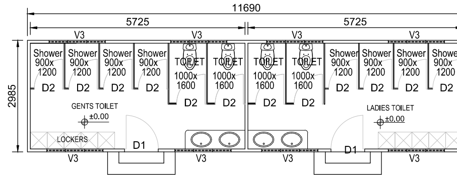
PLAN PLINTH AREA - 34.89 m 2
